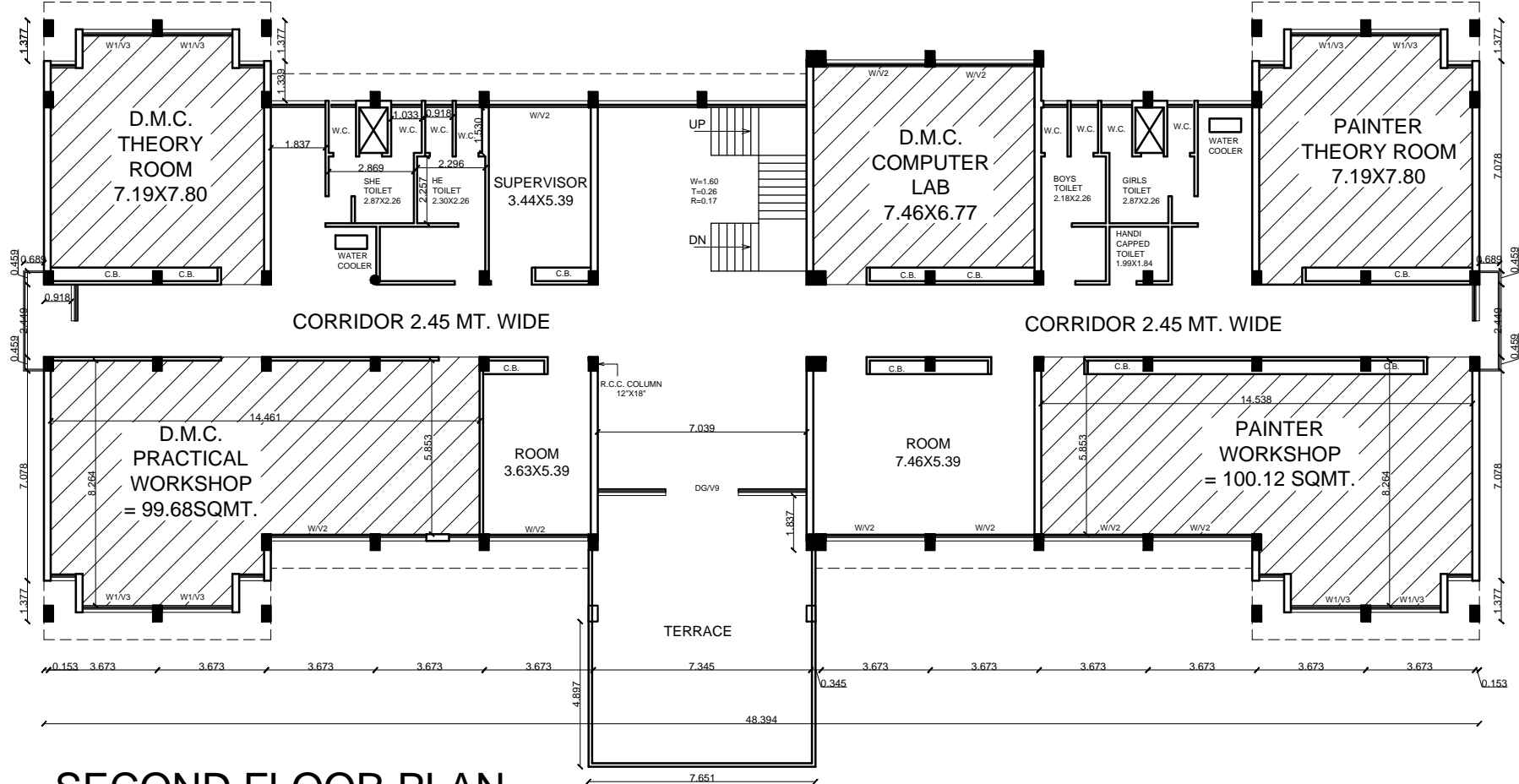
SECOND FLOOR PLAN BLOCK-2
