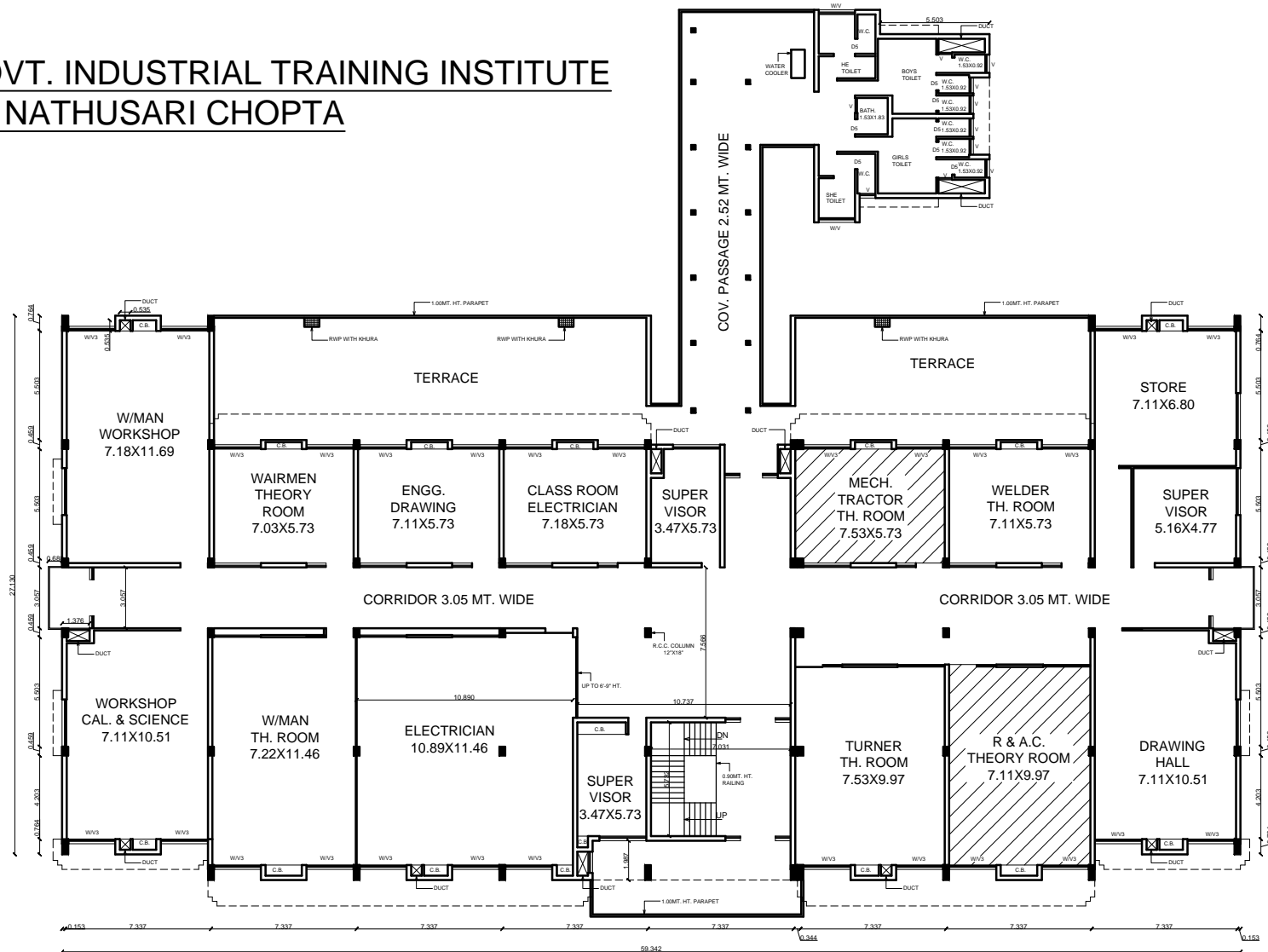
FIRST FLOOR PLAN BLOCK-1
